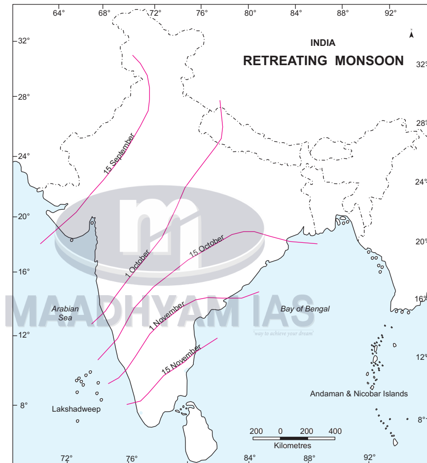
Figure 10.8 Retreating Monsoon
